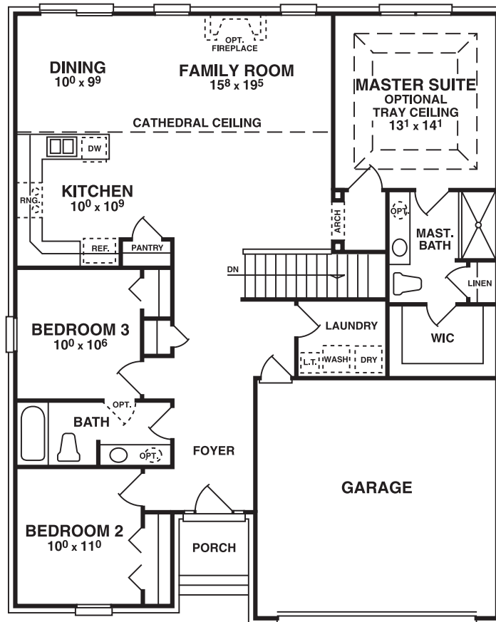
FLOOR PLAN
